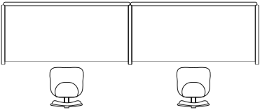
Total Dimensions (L) 2520 x (W) 670 x (H) 1240 mm
